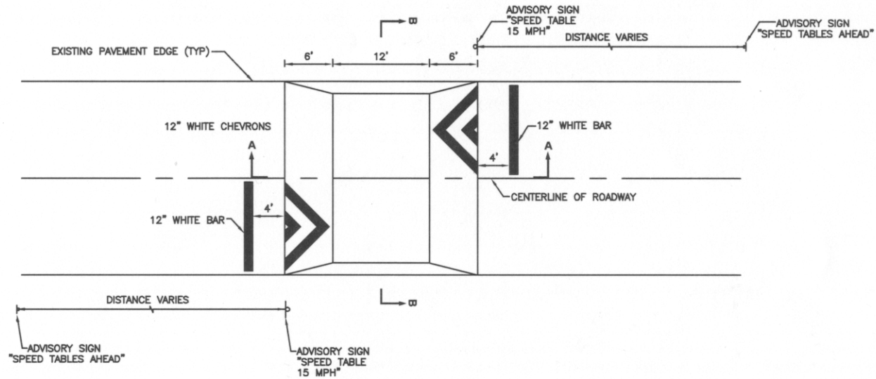
SPEED TABLE TYPICAL LAYOUT
