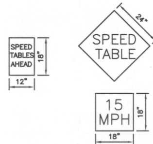
SPEED HUMP TYPICAL SIGNAGE
