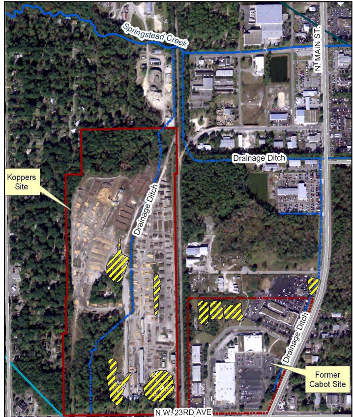
Figure 2.1 Site Layout
